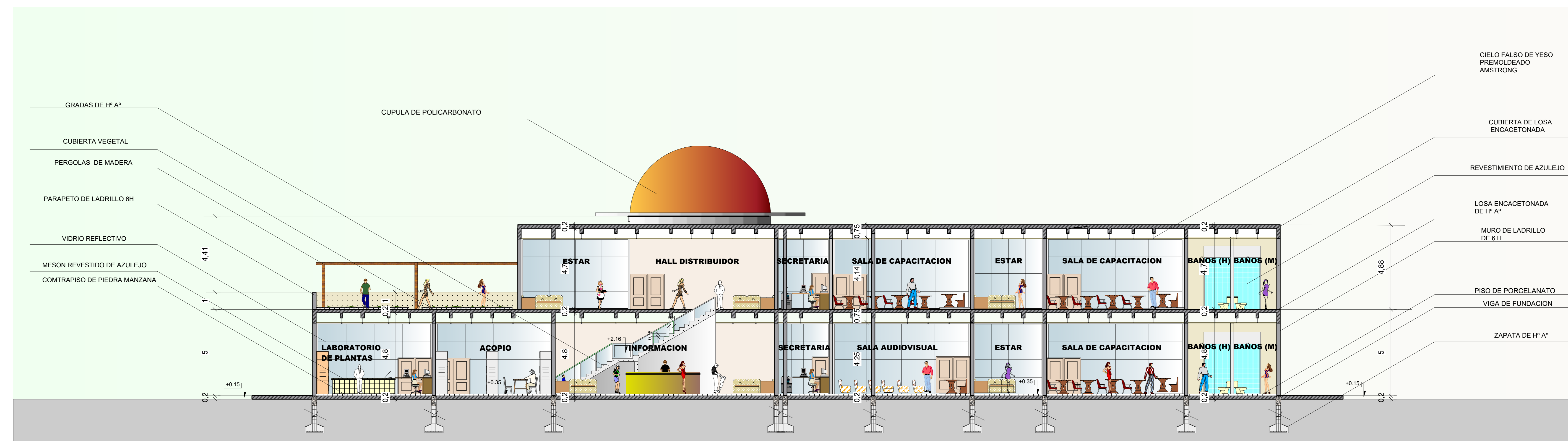
--- CORTE B - B --- ESC: 1:100
