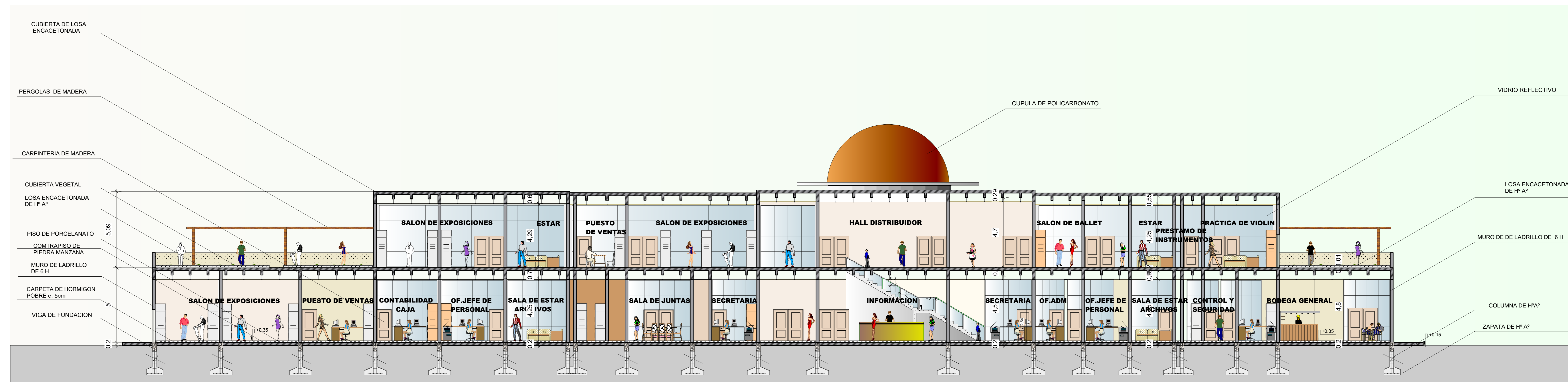
--- CORTE A - A --- ESC: 1:100
