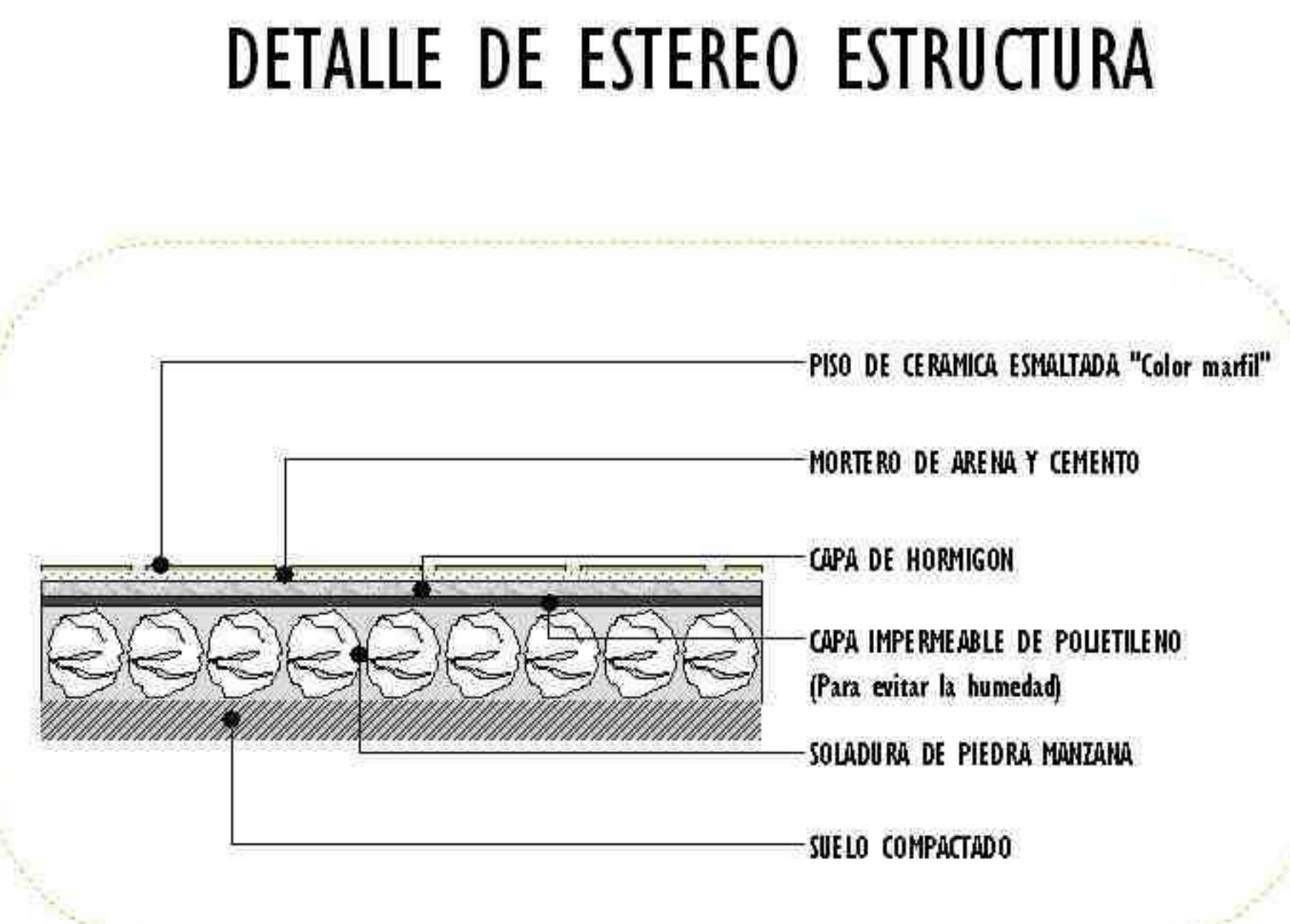
PISO INTERIOR
