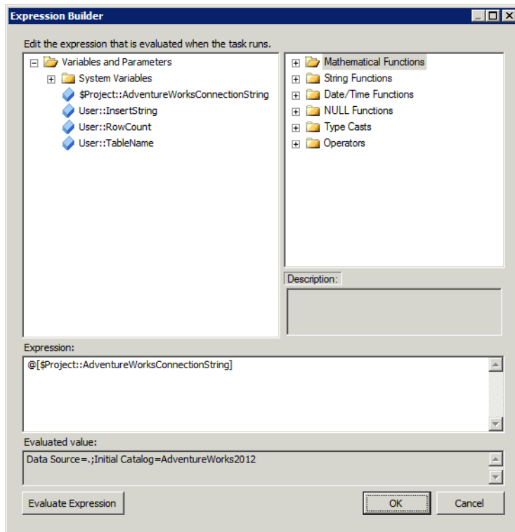
FIGURE 6-20 Parameter usage in an expression
