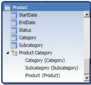
FIGURE 9-9 Hierarchy in the diagram view of a model
