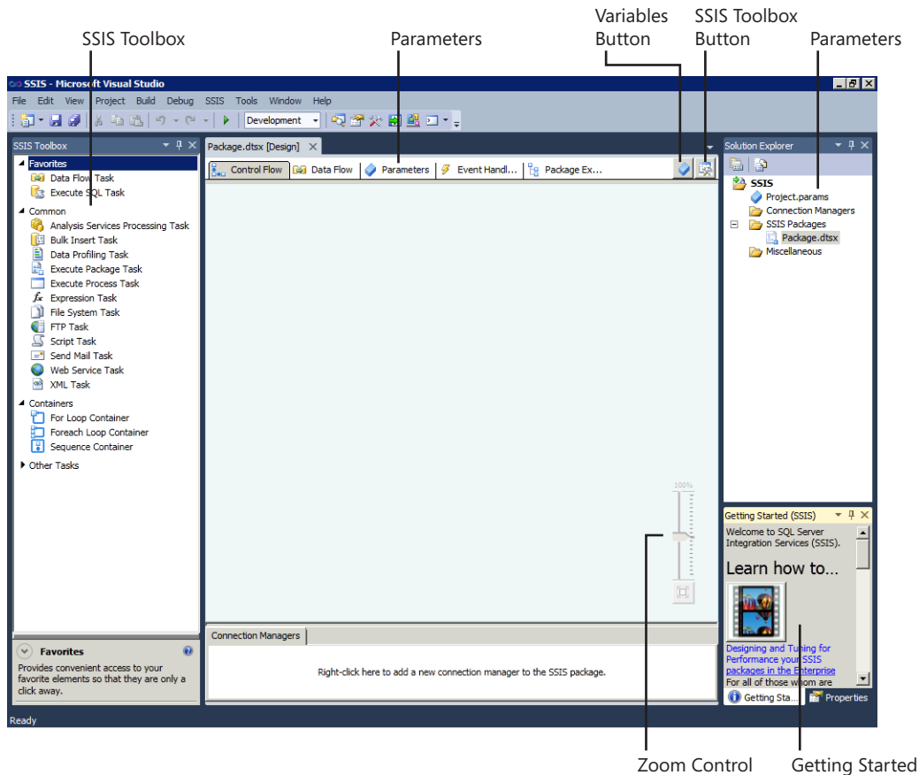
FIGURE 6-2 Package-designer interface changes
