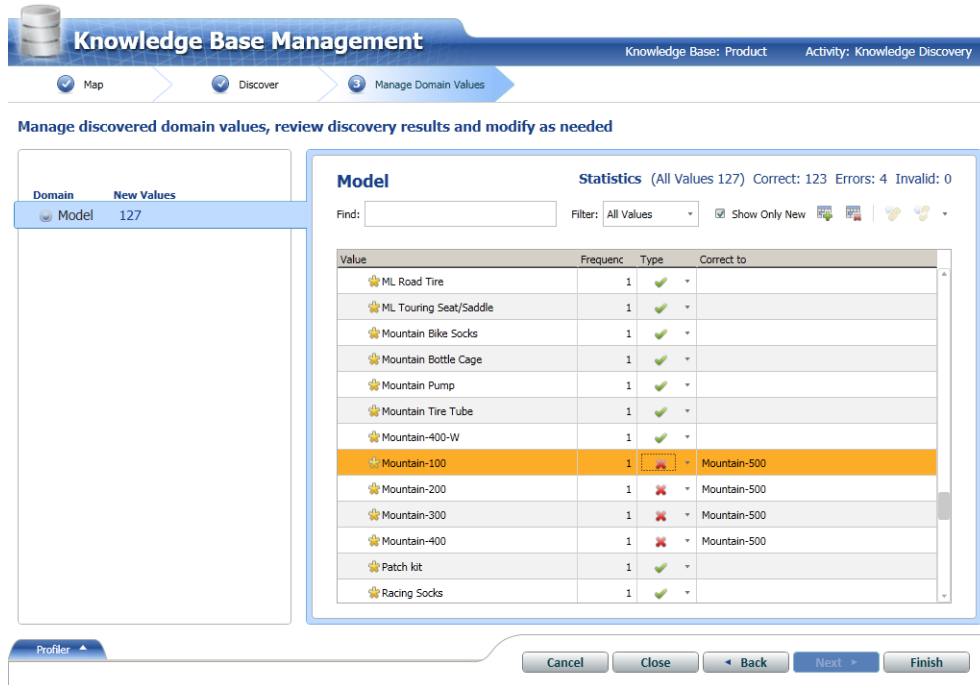
FIGURE 7-14 The Knowledge Discovery activity produces suggested corrections
