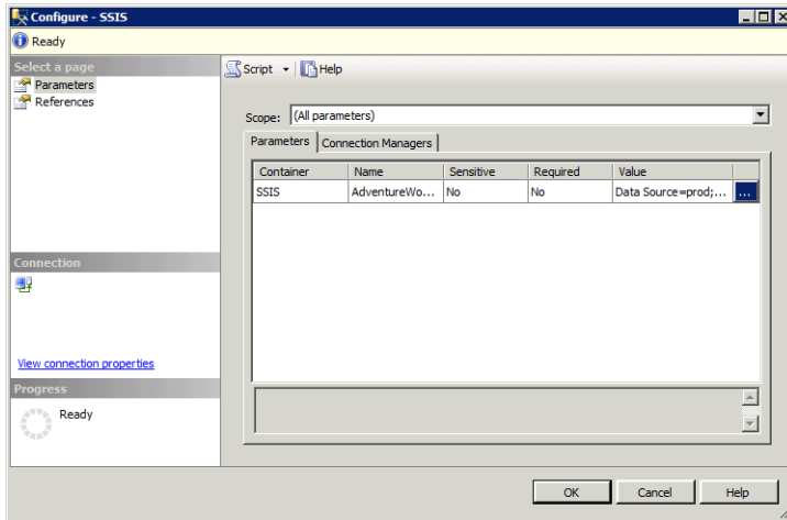
FIGURE 6-23 Server default value configuration
