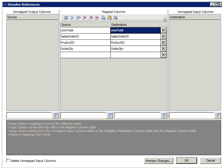
FIGURE 6-11 Resolve References editor for mapping output to input columns
