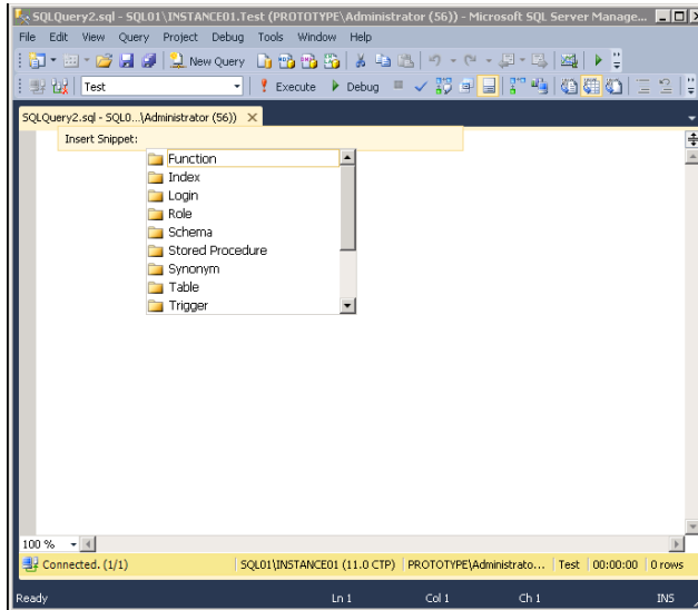
FIGURE 1-4 Leveraging the Transact-SQL code snippet template as a starting point when writing new Transact-SQL statements in the SQL Server Database Engine Query Editor
