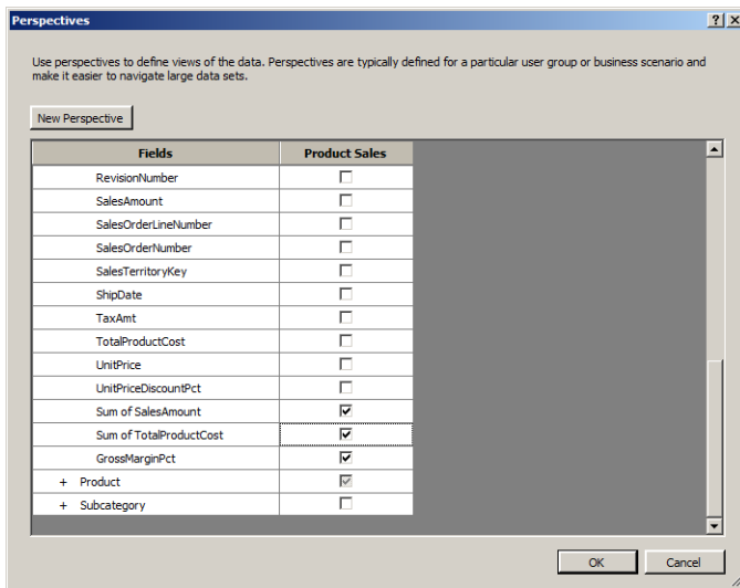
FIGURE 9-10 Perspective definition
