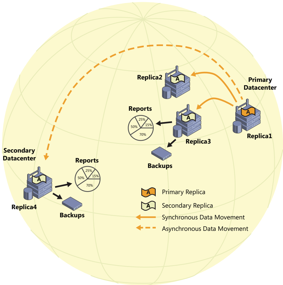
FIGURE 1-2 AlwaysOn Availability Groups for an organization with a global presence
