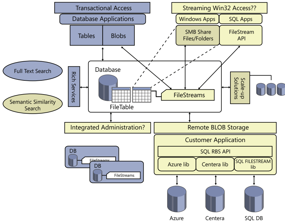
FIGURE 5-1 SQL Server's data and services ecosystem
