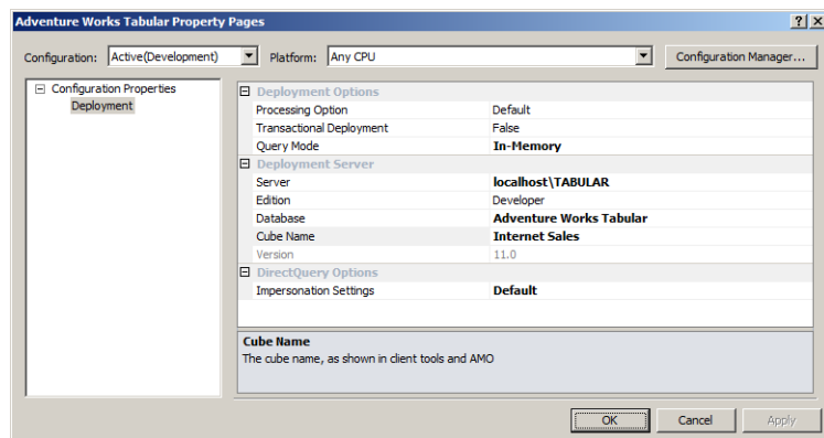
FIGURE 9-13 Project properties for tabular model deployment
