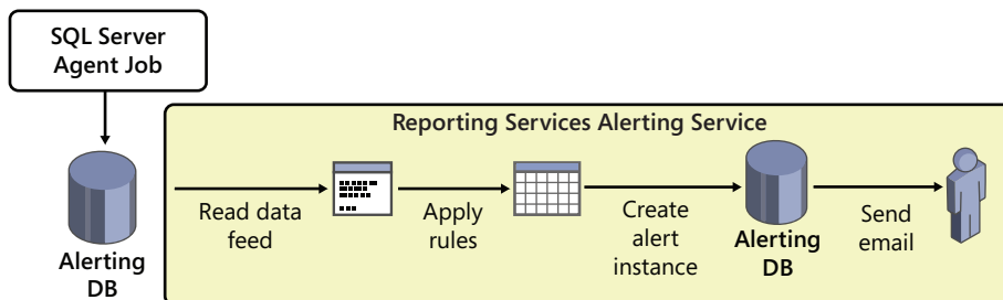
FIGURE 10-23 Alerting service processing of data alerts
