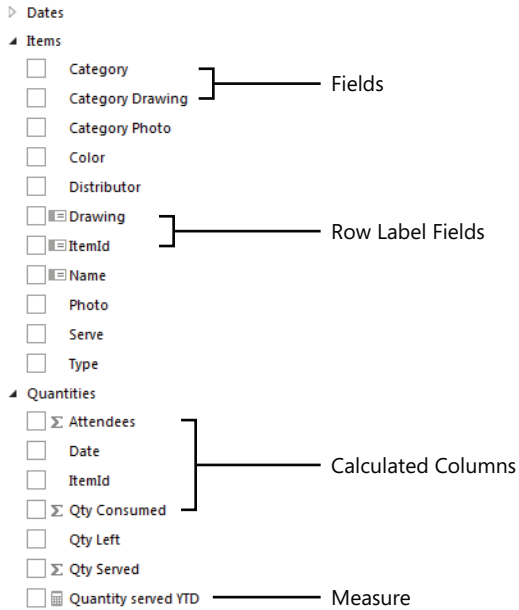
FIGURE 10-3 Tabular model field list
