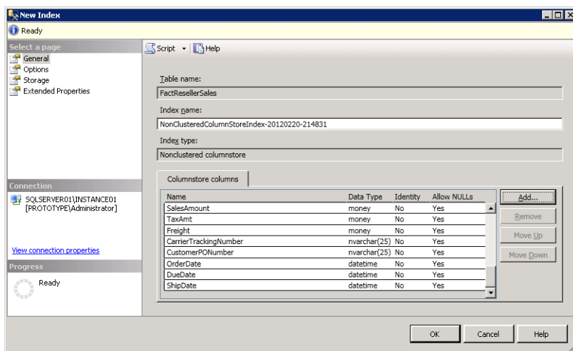
FIGURE 3-3 Creating a nonclustered columnstore index with SSMS
