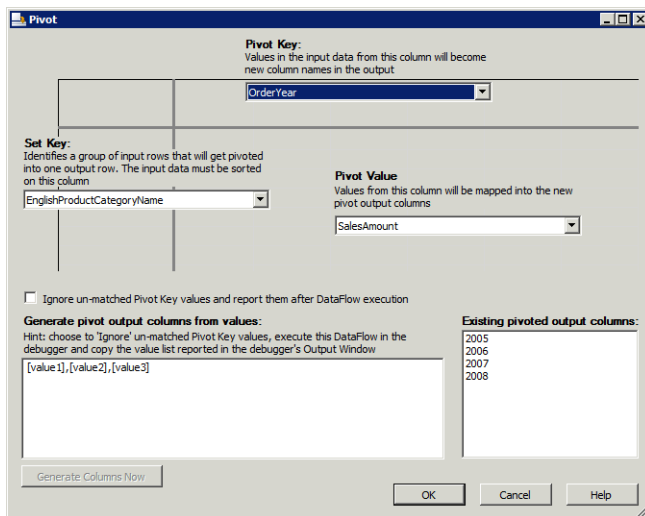
FIGURE 6-9 Pivot transformation editor for converting a set of rows into columns of a single row
