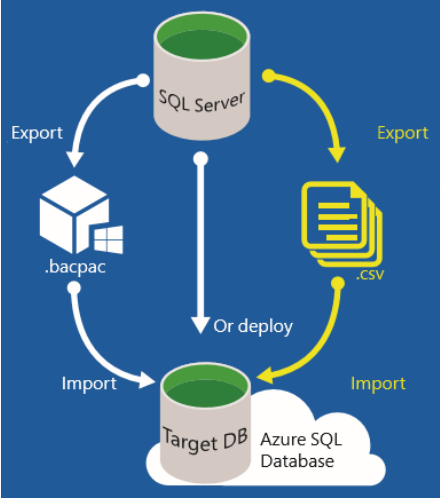
Figure 4-2: SQL Database import processes for compatible databases
