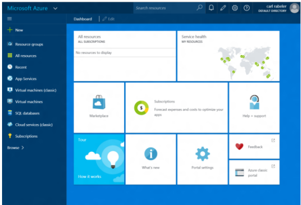
Figure 1-2: Azure portal
