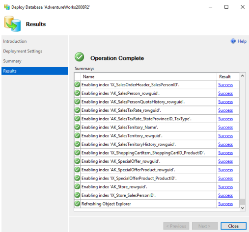
Figure 4-38: Migration complete
