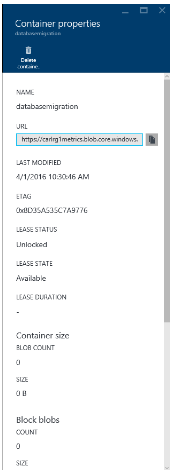
Figure 4-14: Container properties
