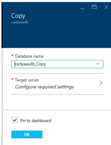
Figure 5-31: Copy blade
