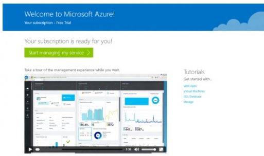
Figure 1-10: Subscription complete
