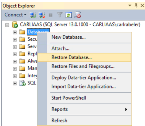
Figure 4-20: Restore database
