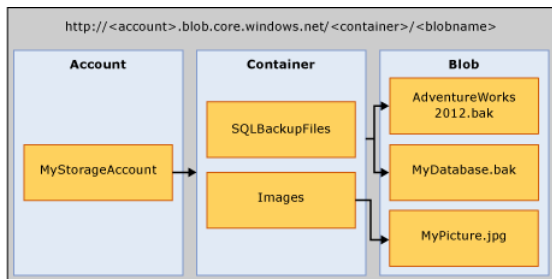
Figure 5-6: Backup to URL architecture
