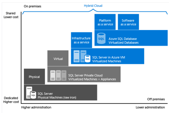
Figure 1-1: IaaS vs. PaaS vs. SaaS
