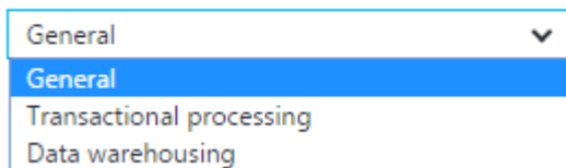
Figure 2-26: Storage optimization
