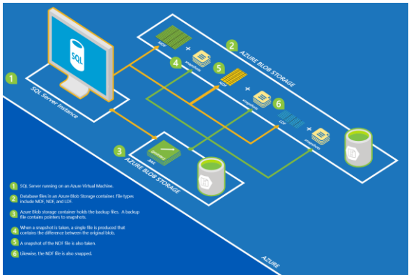
Figure 5-7: File-snapshot backup architecture
