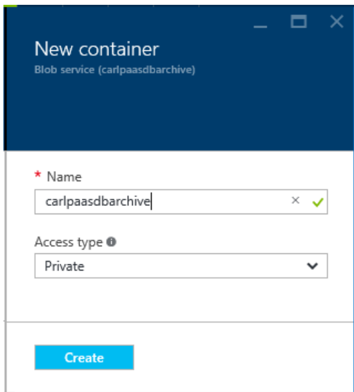
Figure 5-46: New container
