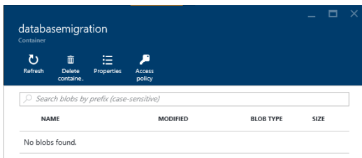
Figure 4-13: New container
