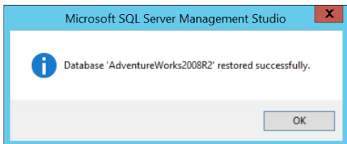
Figure 4-24: Restore success
