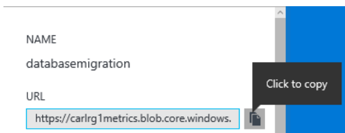
Figure 4-15: Copy URL
