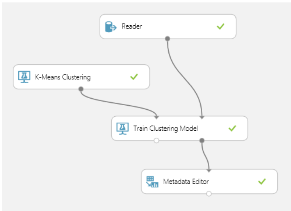
FIGURE 6-14 The K-means clustering experiment for analyzing wholesale customers in Azure ML Studio.
