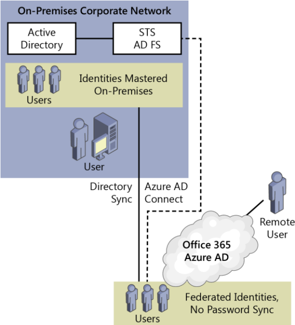
Figure 2-4: An overview of federated identities.
