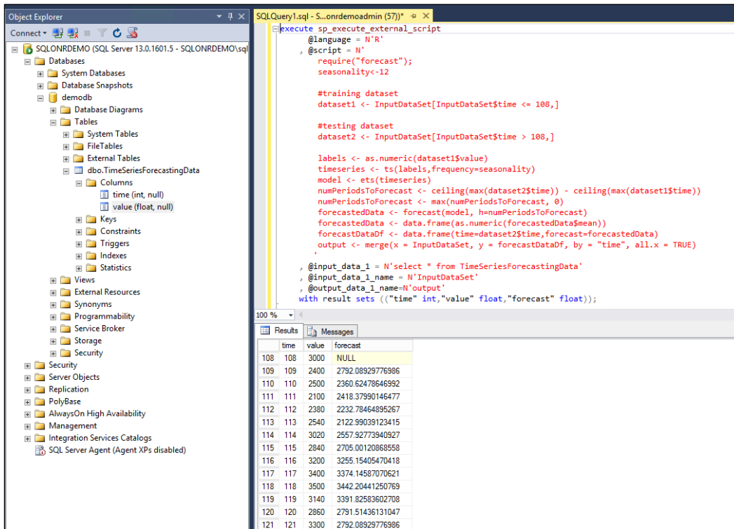
Figure 6-6: SQL Management Studio with the query and expected output after the query has been run. Now three columns are displayed: time, value, and forecast.
