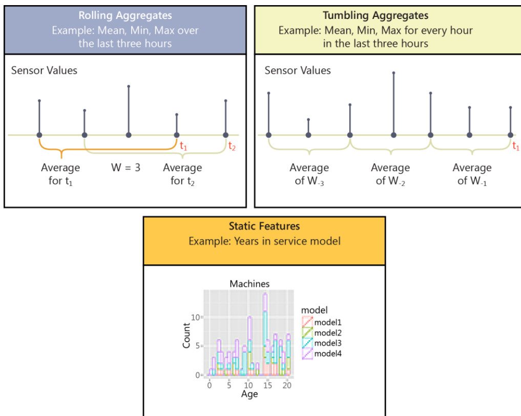
Figure 5-8: An example of features to be included in the model. 11
