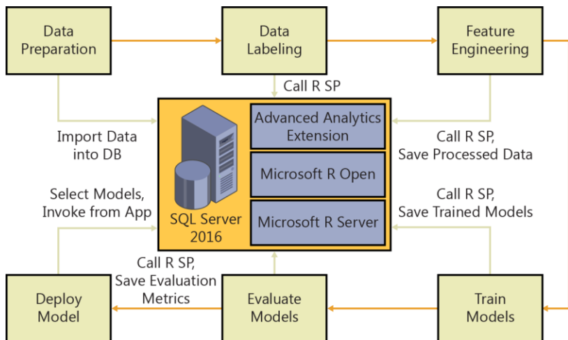
Figure 5-10: Workflow automation. 13
