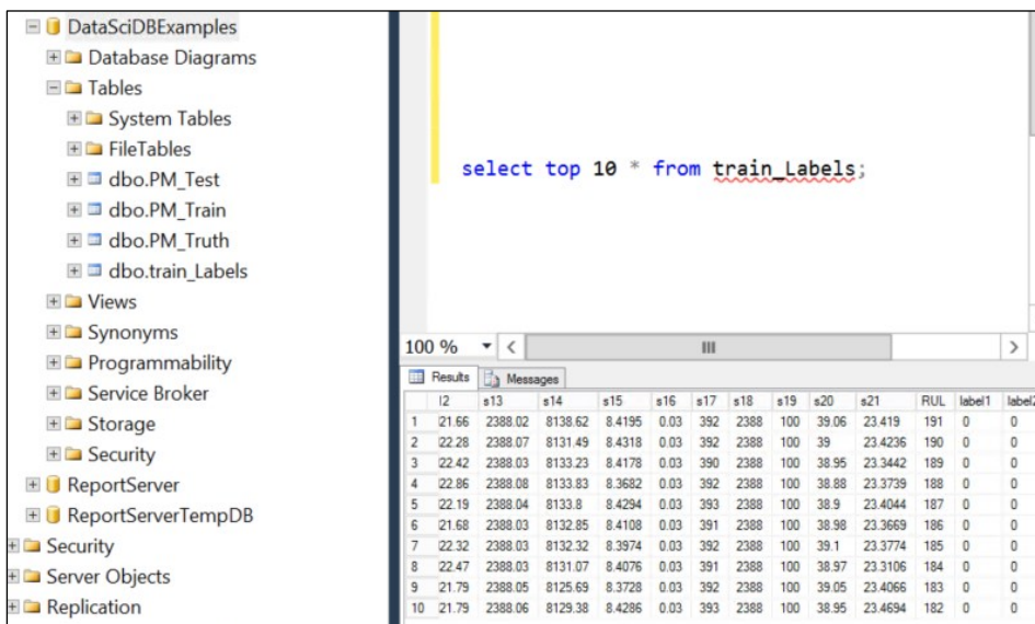
Figure 5-7: View of database tables using Microsoft SQL Server Management Studio.
